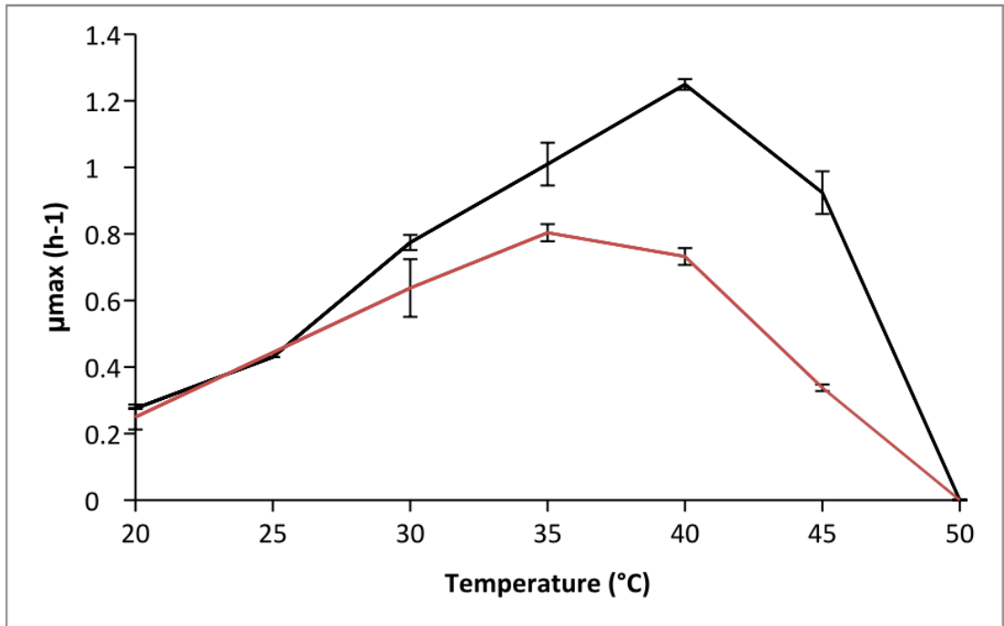
Figure 1 - Temperature optima of strain CC5C (black line) and E. coli (red line, DSM 30083) grown in TSB. Values represent average of triplicates with the standard deviation presented as error bars.
